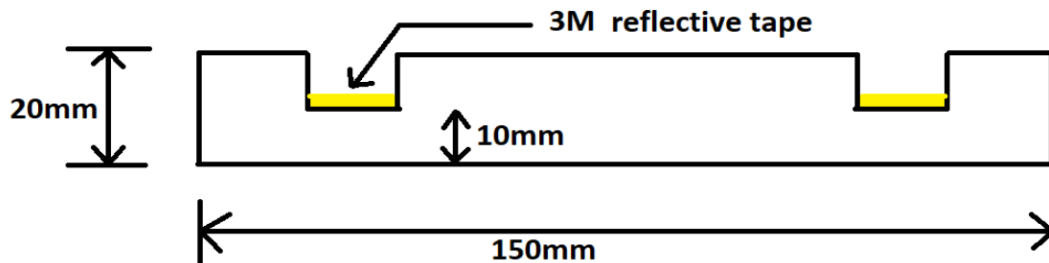
(Indicative Drg. of Rubber Stopper)
